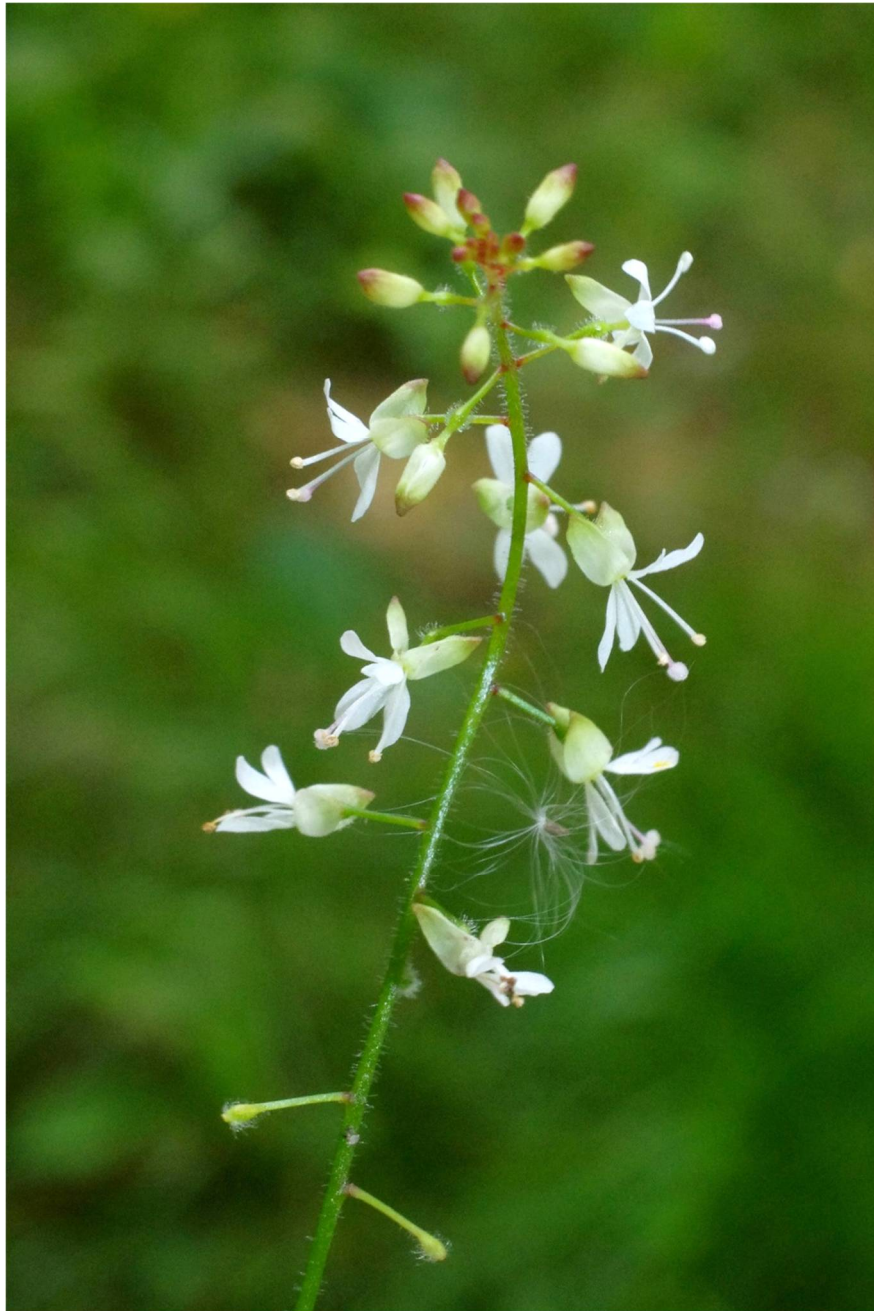
Circaea x intermedia
