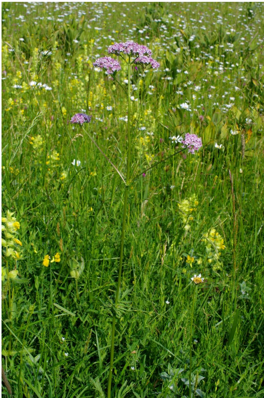
Valeriana pratensis subsp. angustifolia Ioannina, NW Metsovo, 1380 m, 39°47'04"N, 21°09'33"E, 15.06.2017; 276.743
